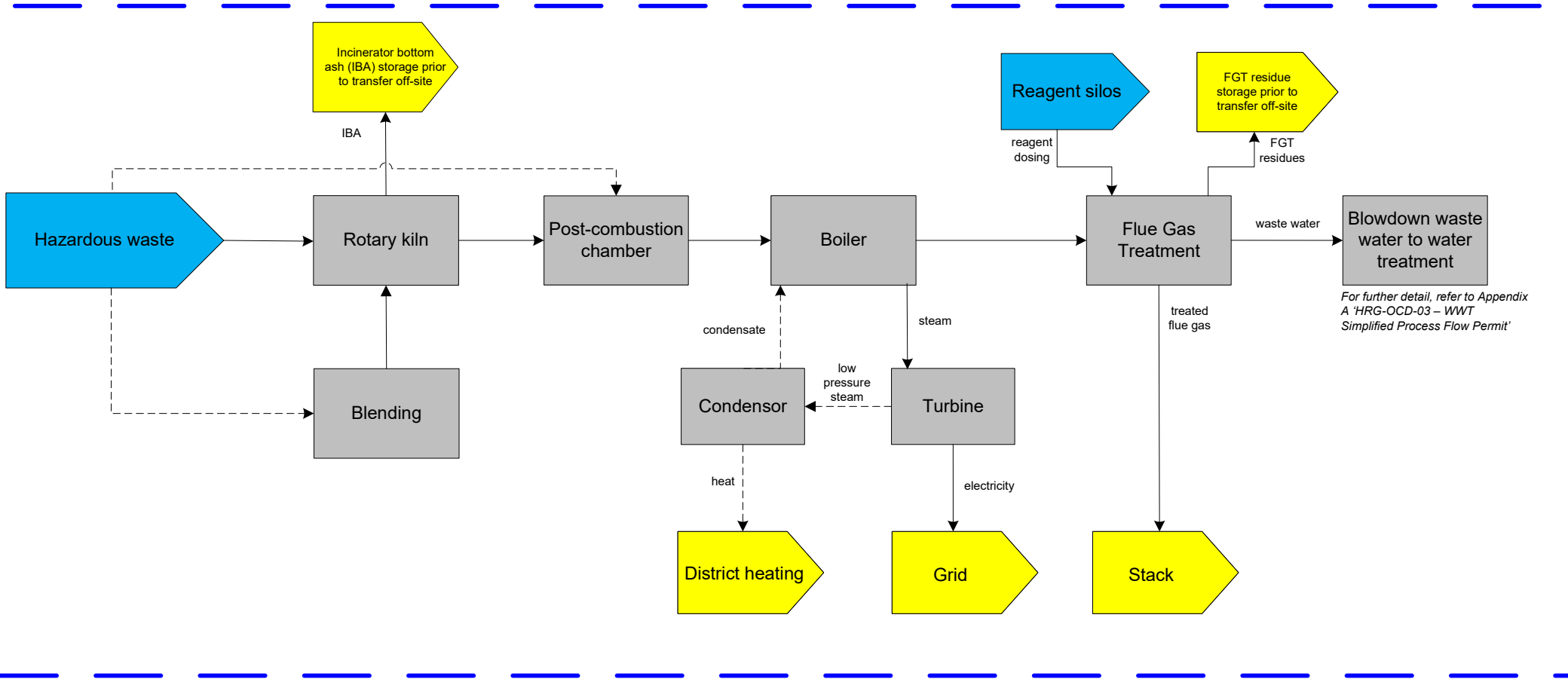
Indicative Process Diagram
