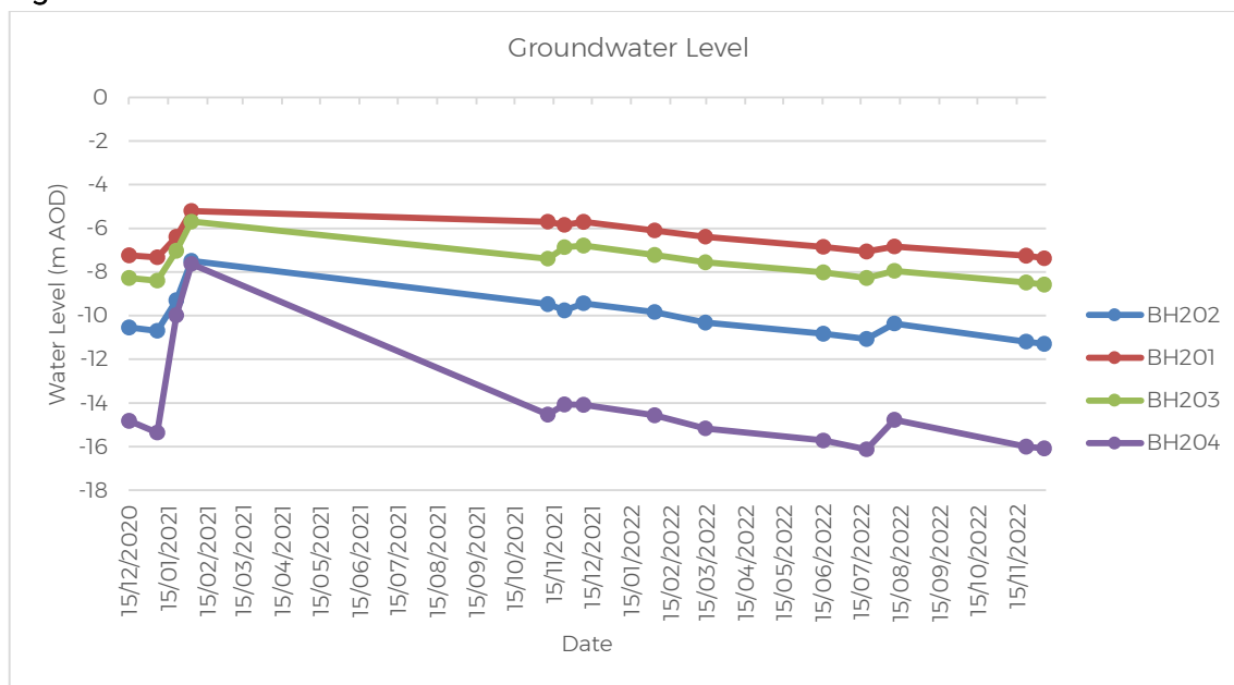
Figure 4: Groundwater Levels
