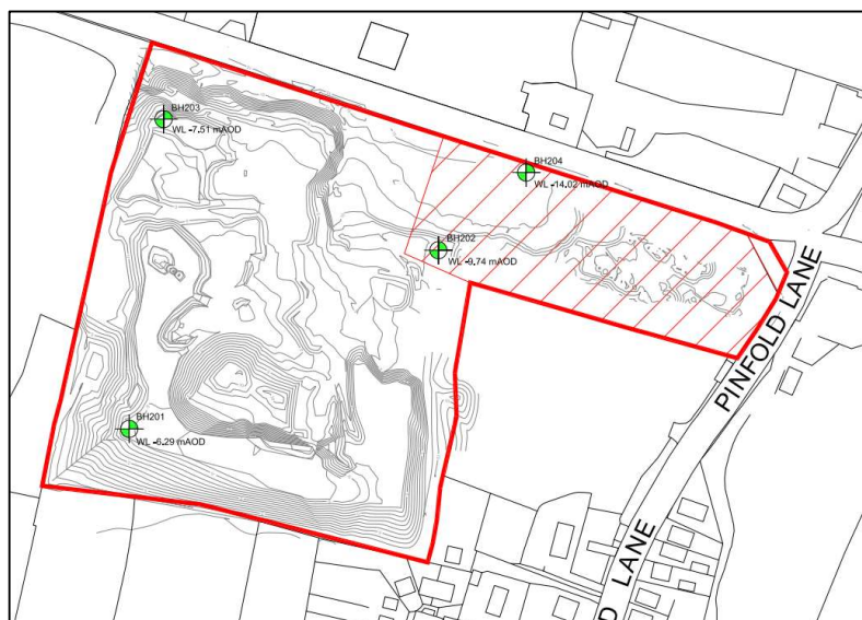
Figure 1B: Site Plan (taken from AAe drawing 163407/BH/002)
