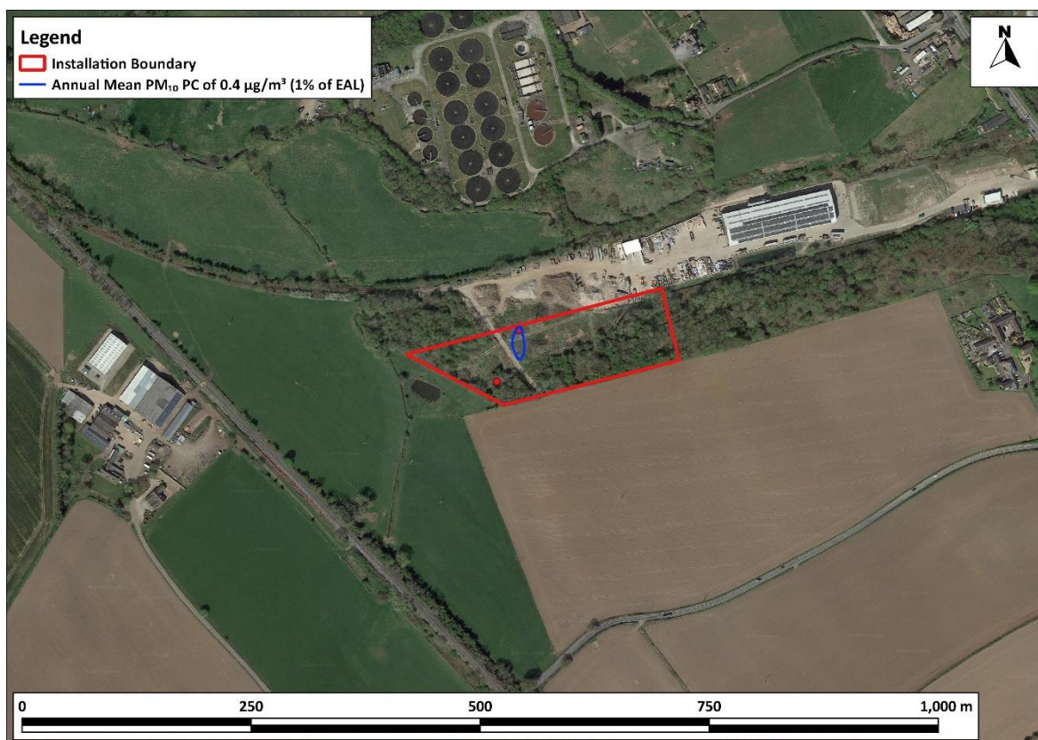
Figure 12: Annual Mean \text{PM}_{10} Process Contributions from the Generator (Ground Level)
