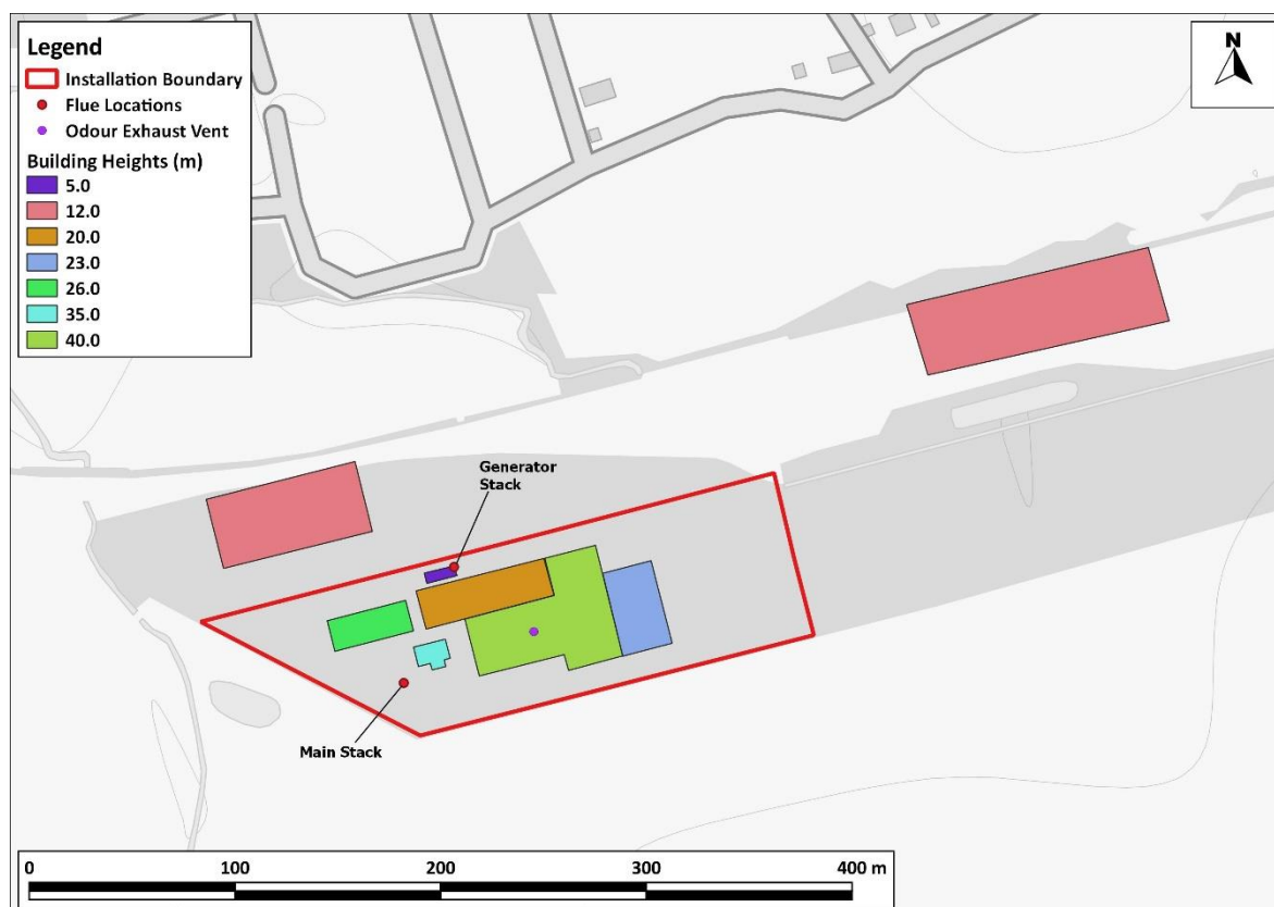
Figure 4: Site Layout
