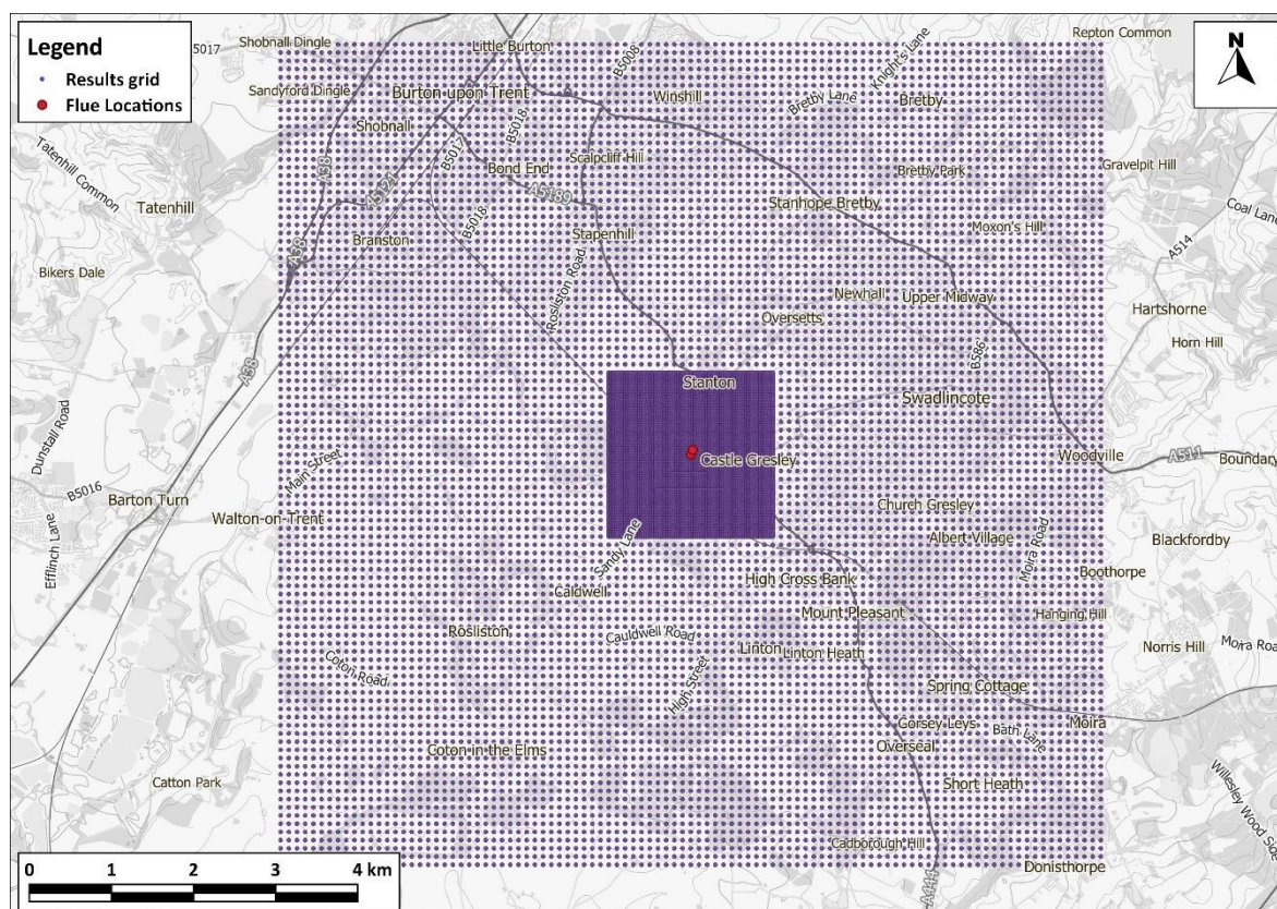
Figure 6: Modelled Receptors Nested Grid
