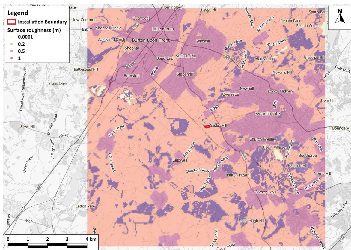
Figure 8: Surface Roughness across Modelled Area
