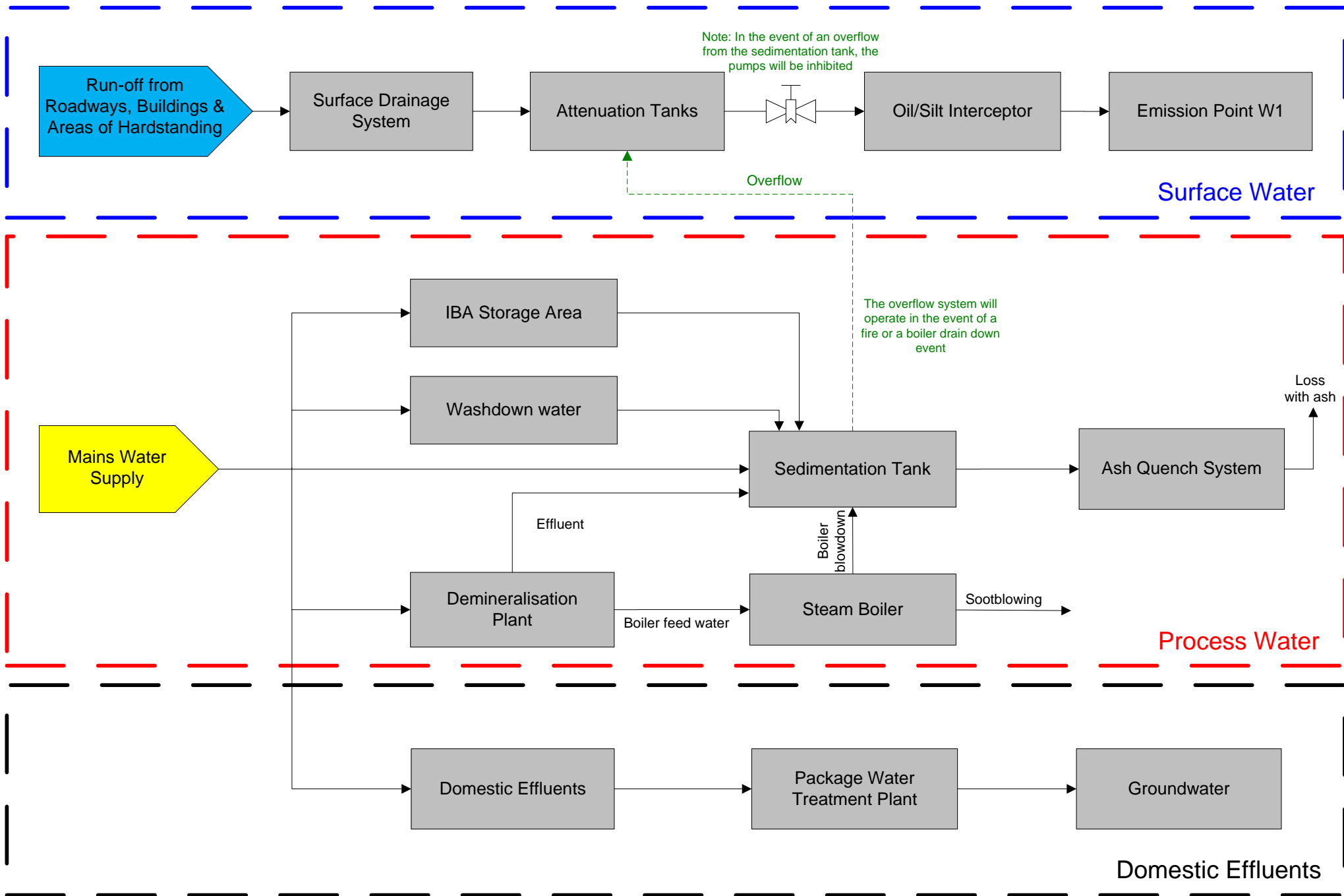
Figure 3 – Indicative Water Flow Diagram
