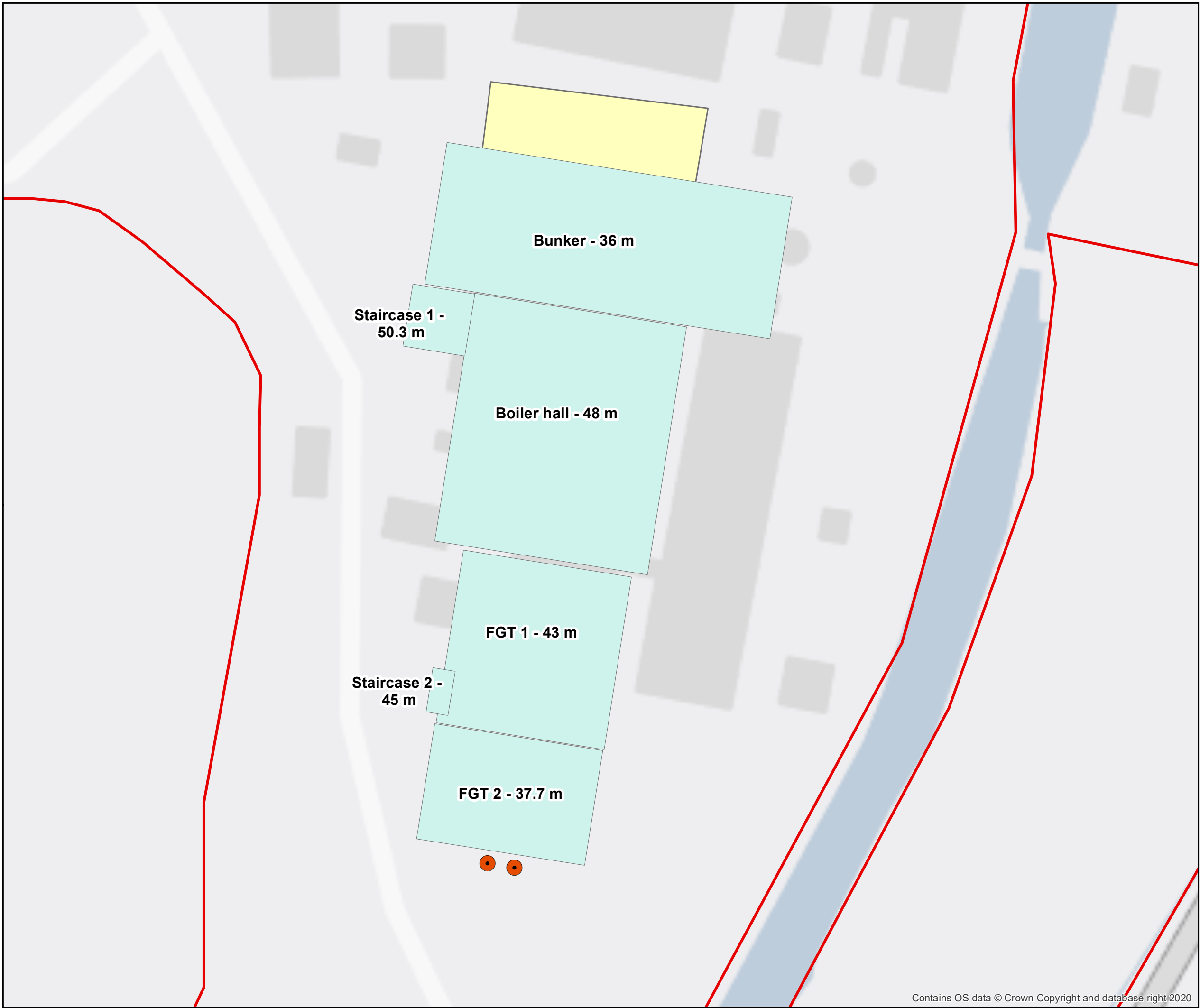
Figure 4 - Proposal buildings
