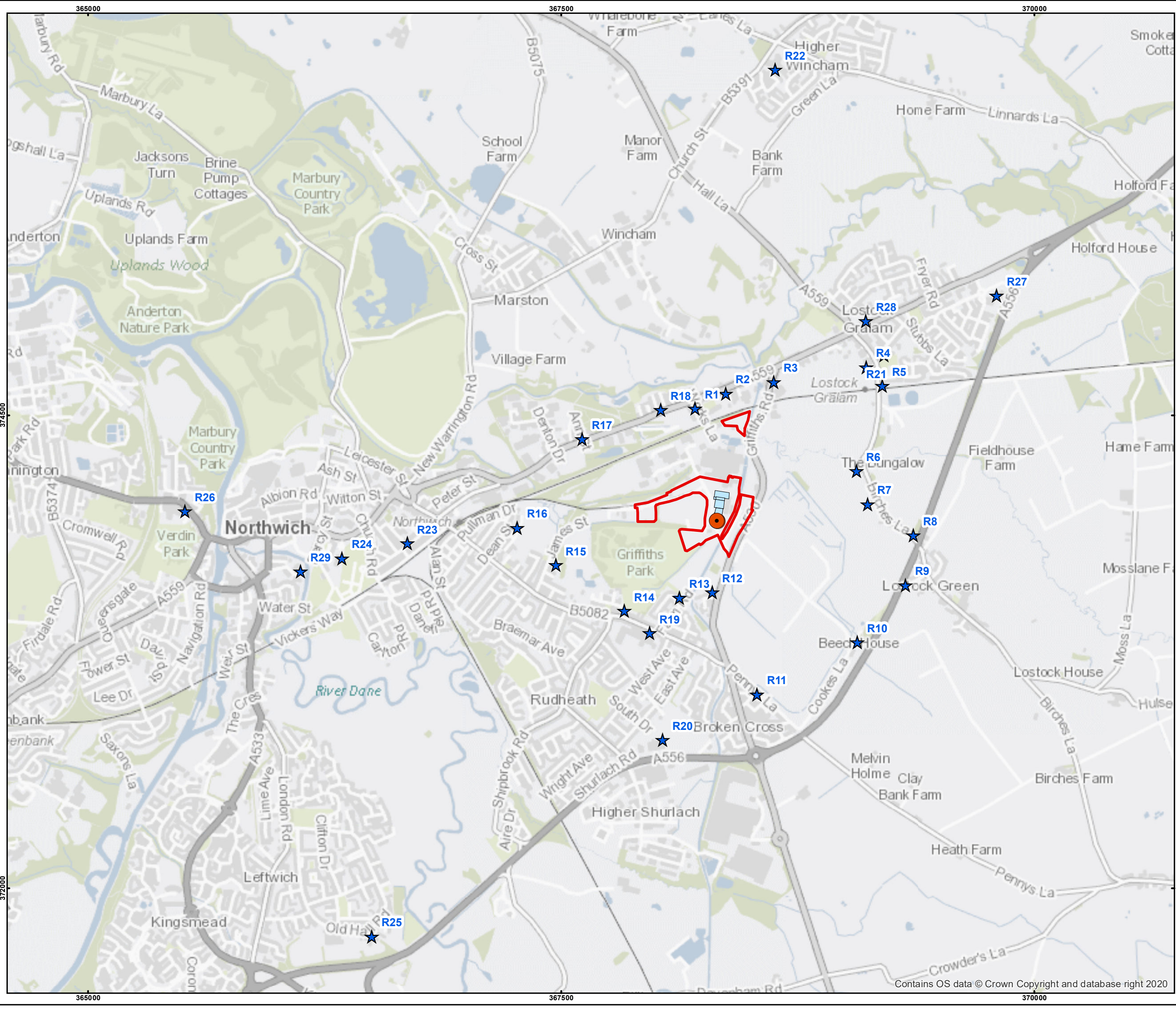
Figure 5.2 - Human receptors
