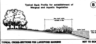
TYPICAL CROSS-SECTIONS FOR LAKE/POND MARGINS NOT TO SCALE
