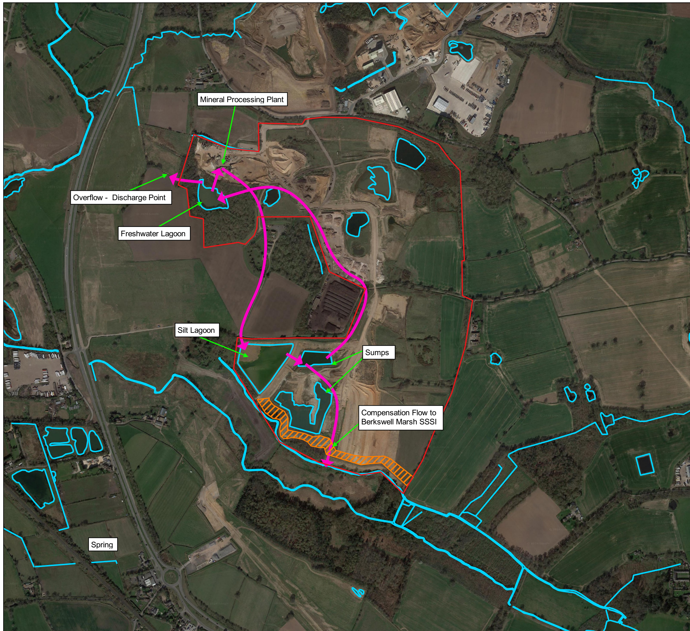
FIGURE 2B Surface Water Management
