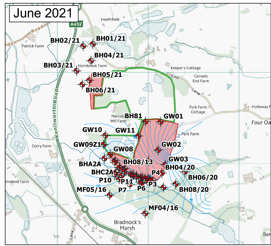
FIGURE 3 Groundwater Contour Plots, 2021
