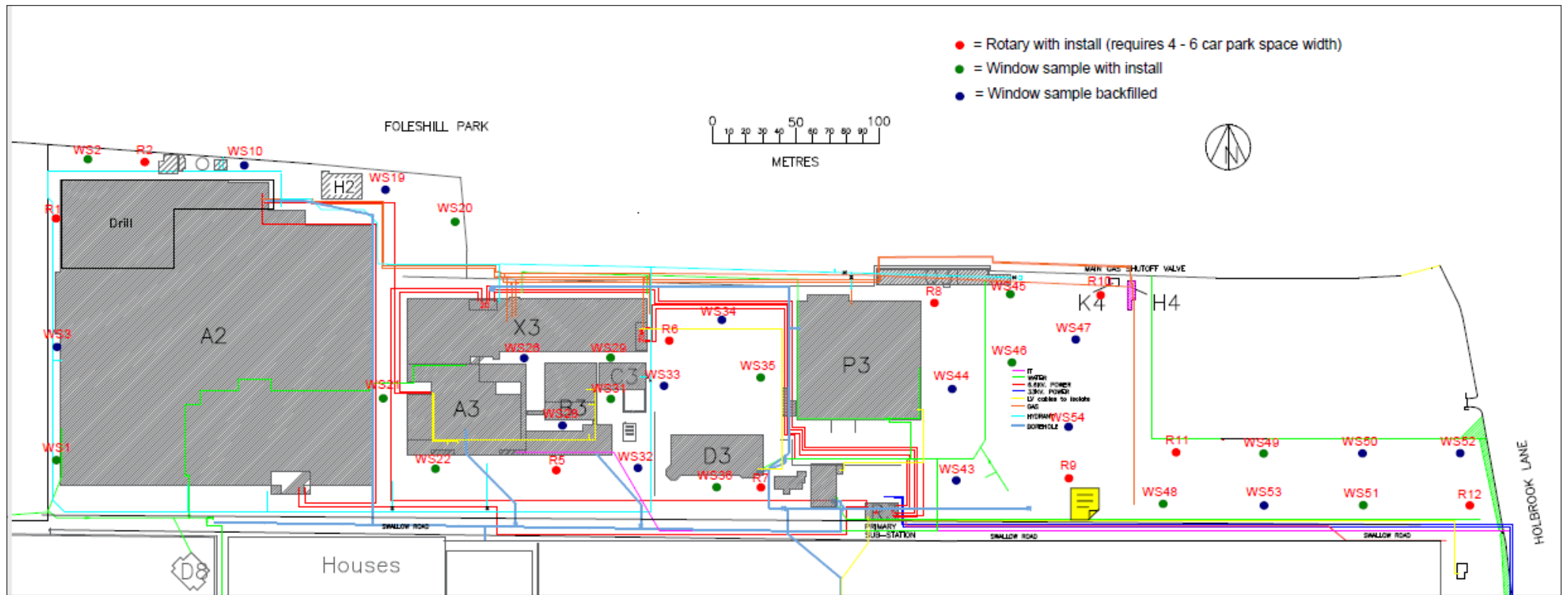
Figure 2: Exploratory Hole Location Plan
