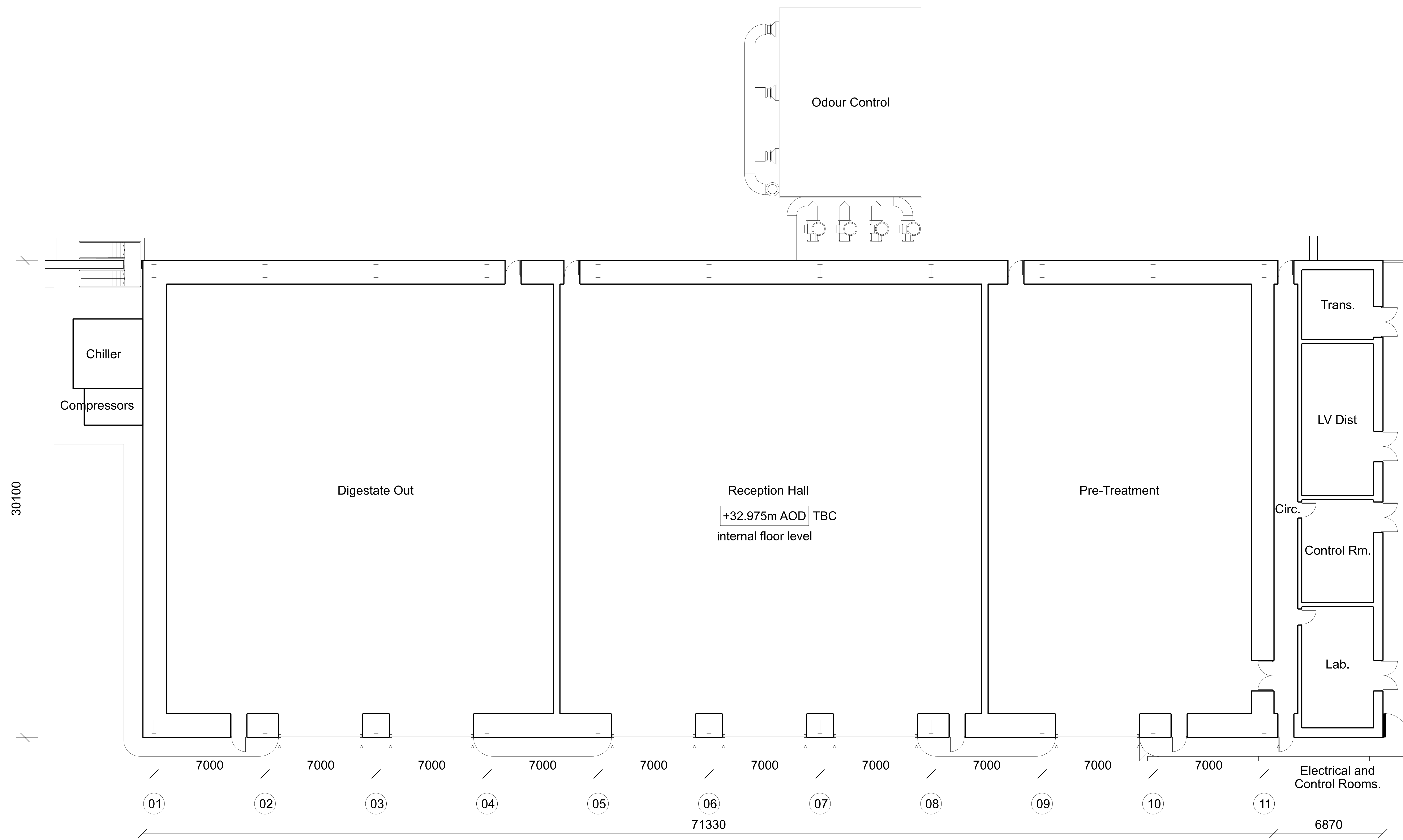
Proposed Floor Plan
