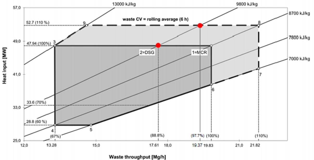
Figure 1: Firing diagram
