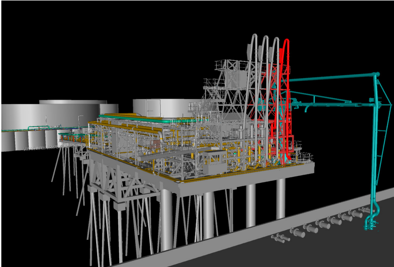
Marine loading arm (located on South Jetty) in the operating position at high tide. Marine loading arm is shown in turquoise.
