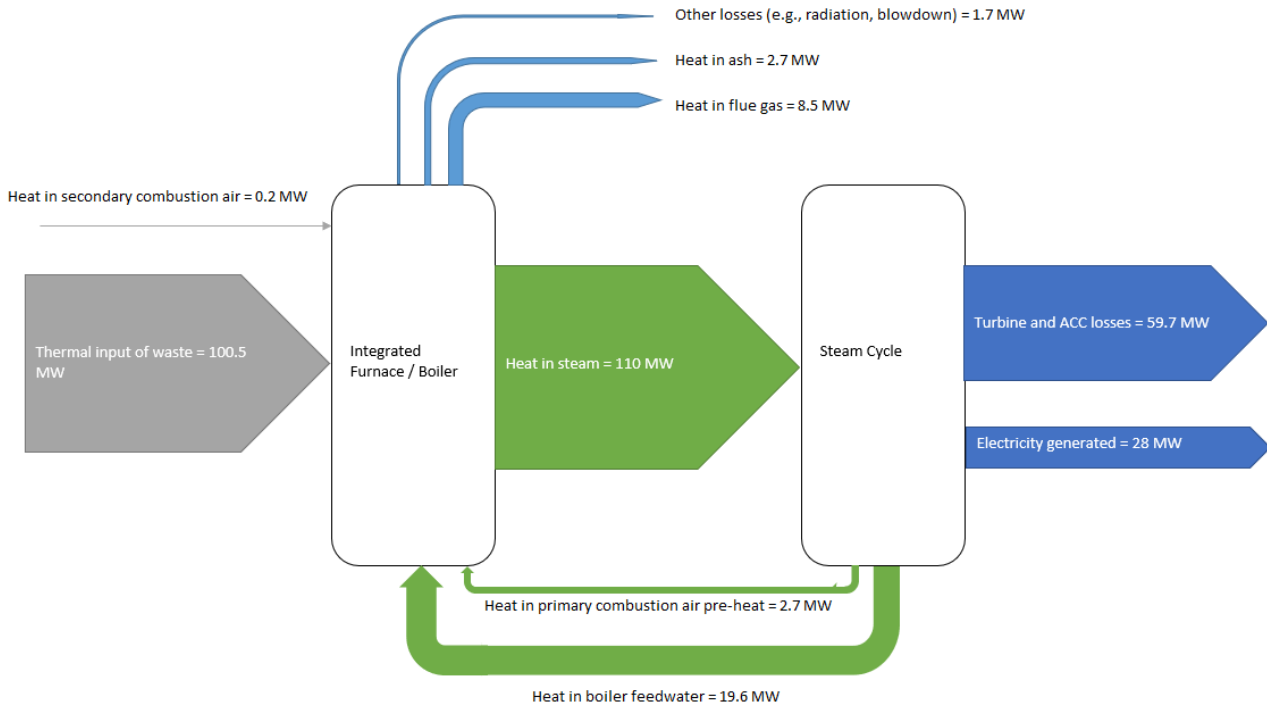
Figure 3-2 Indicative Sankey diagram for energy flows
