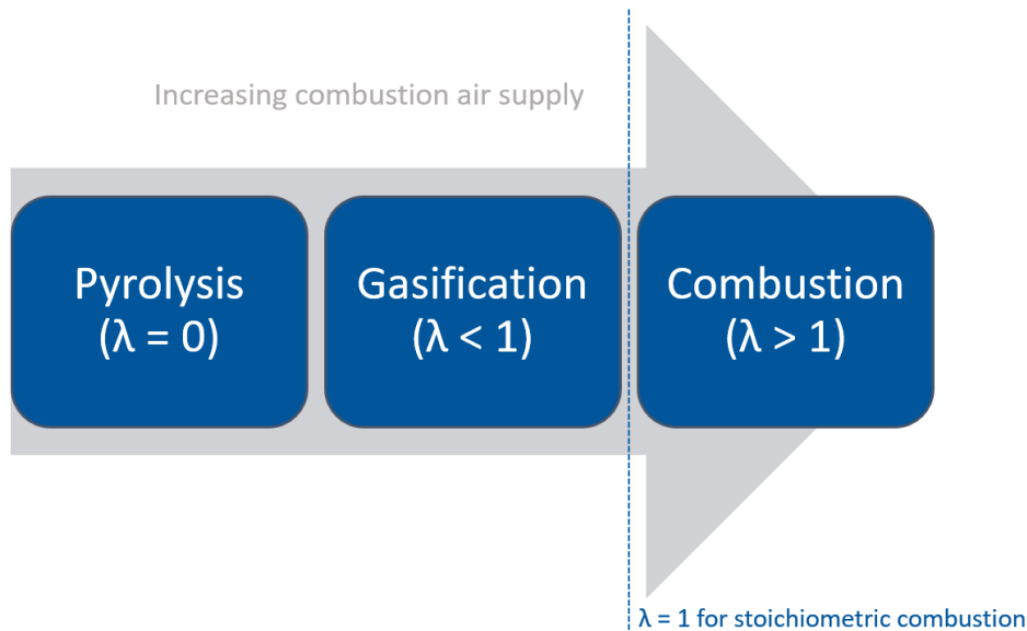
Figure 4-3 Air/fuel ratios for different thermal treatment techniques
