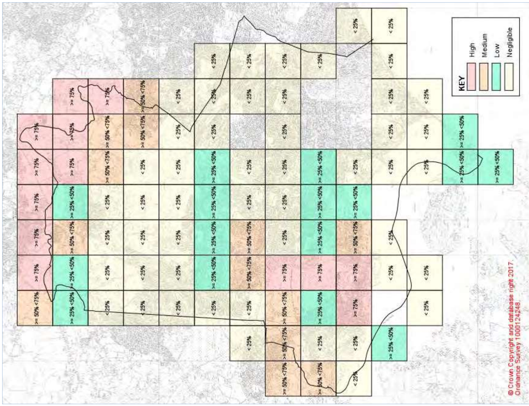
Figure 6: Areas susceptible to groundwater flooding.
