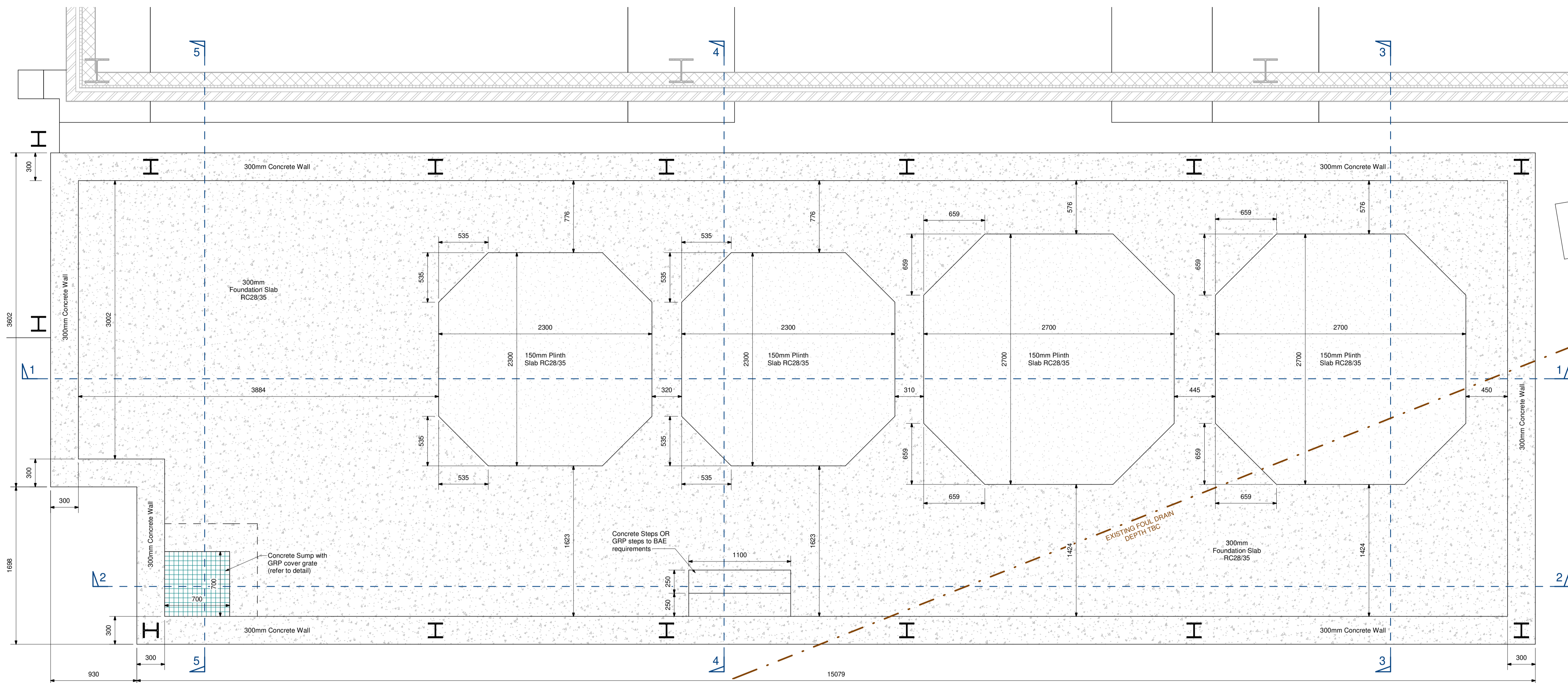
1 NEW BUND GENERAL ARRANGEMENT 1 : 25
