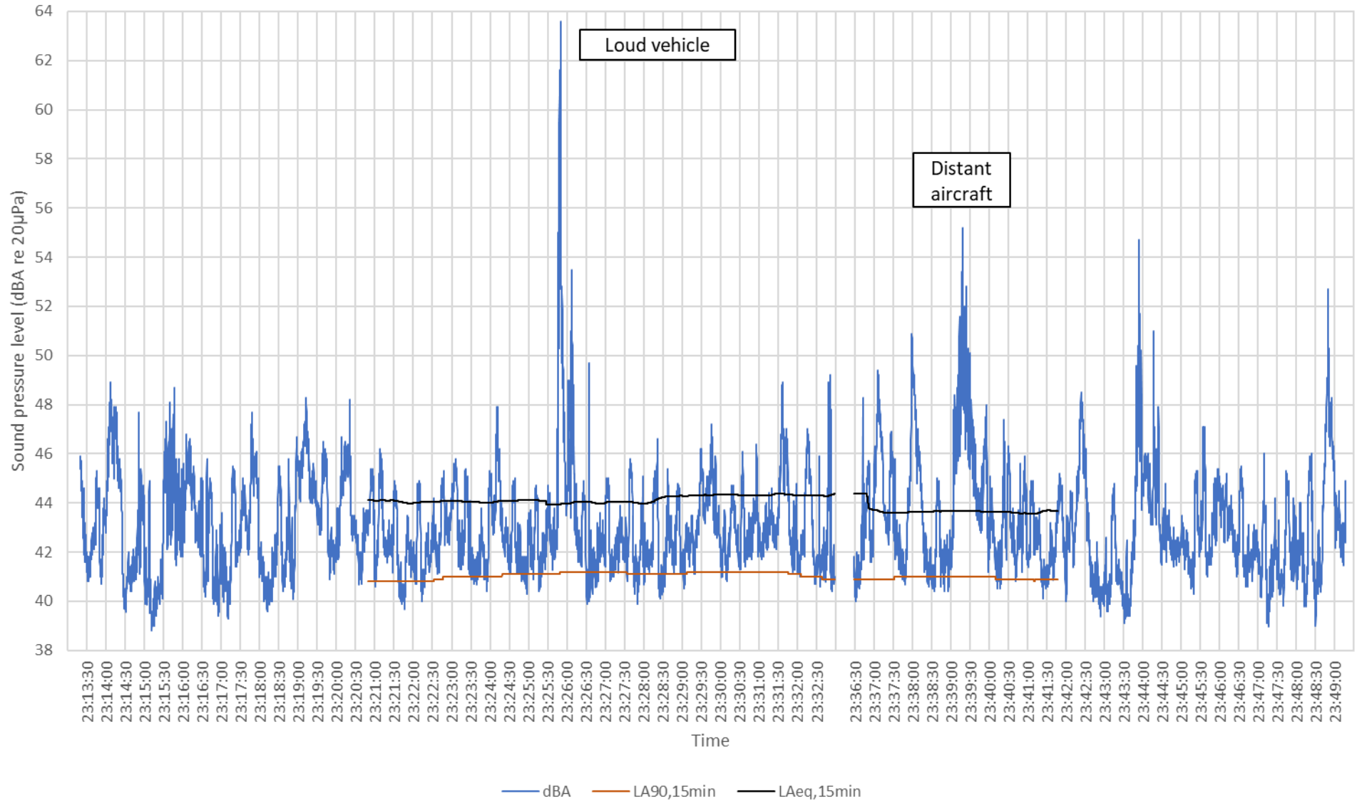
Graph 2 - Ambient sound level to rear of dwellings Measured 13 th April 2023
