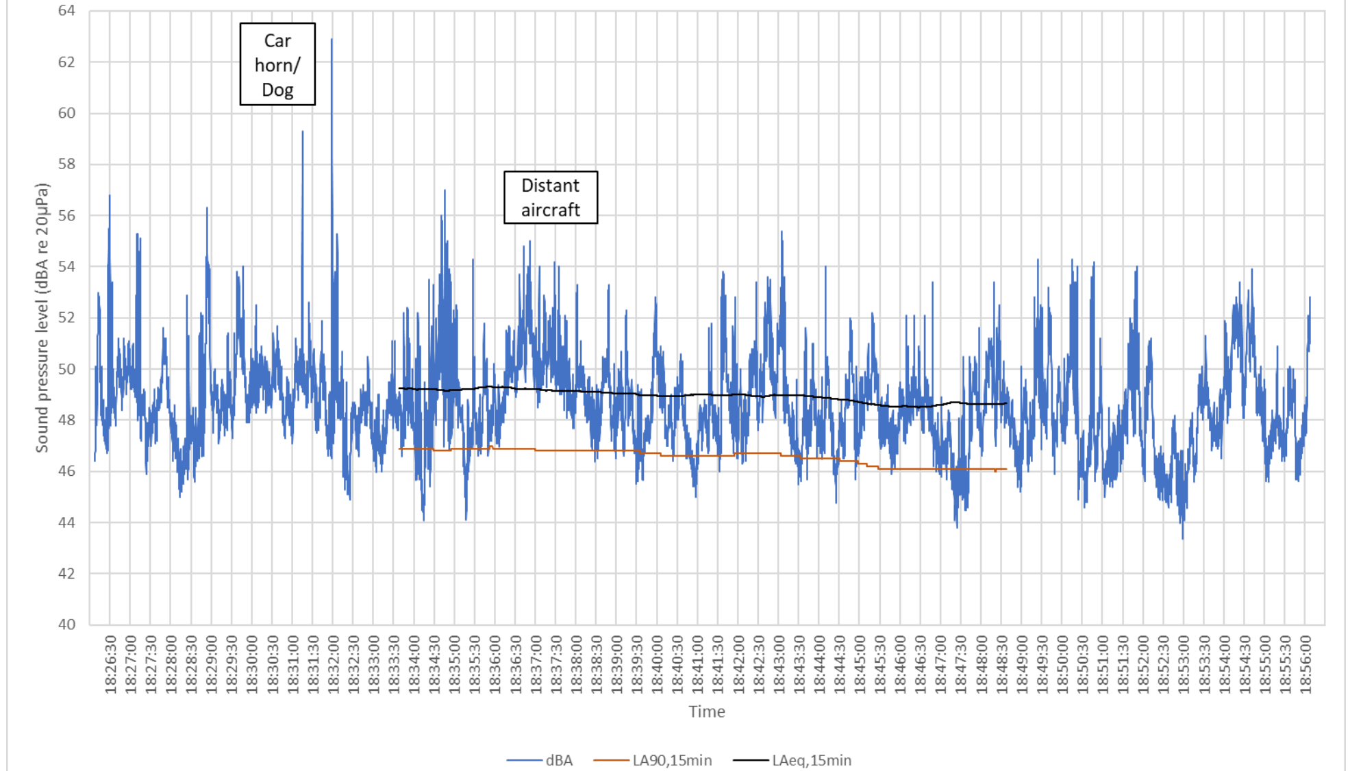
Graph 1 - Ambient sound level to rear of dwellings Measured 13 th April 2023
