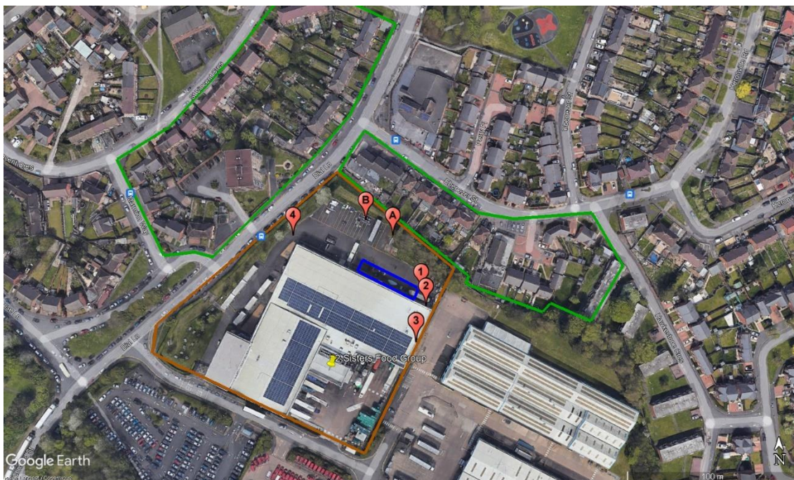
Figure 7.1 Site, Receptors, Plant, and Measurement Locations
