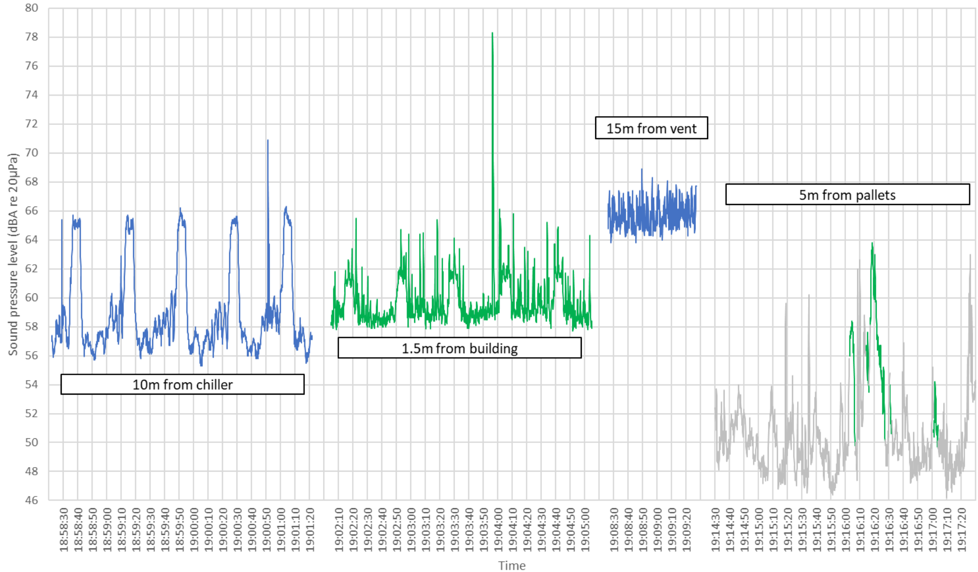
Graph 3 - Ambient sound level near to specific sources Measured 13 th April 2023
