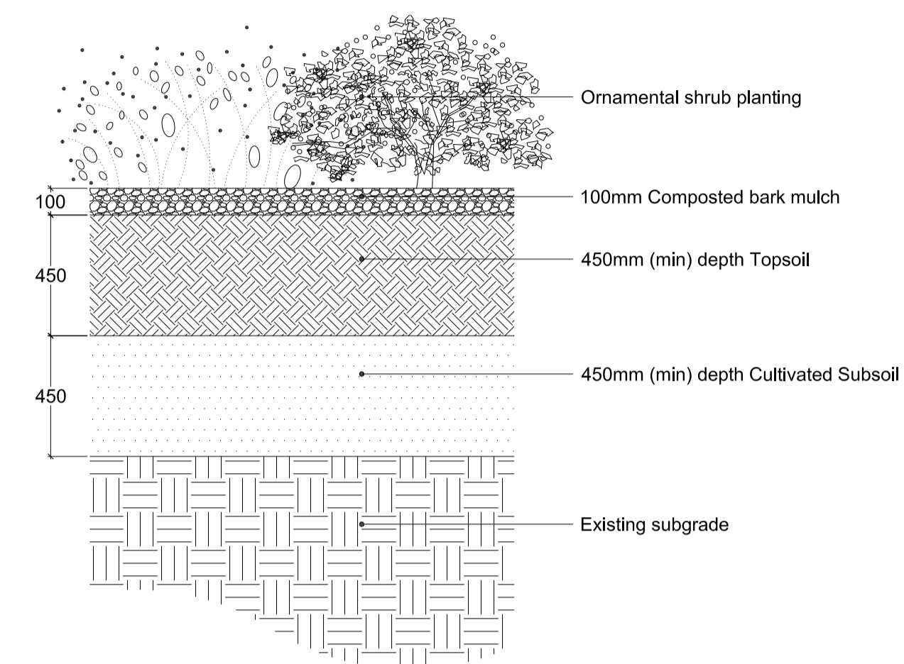
G Typical Shrub Planting Detail Section 1:20@A1
