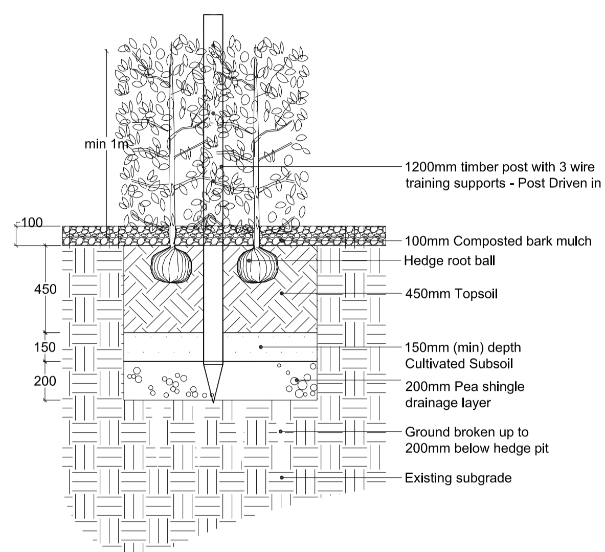
F Typical Native Hedge Planting and Post and Wire Fence Detail Section 1:20@A1
