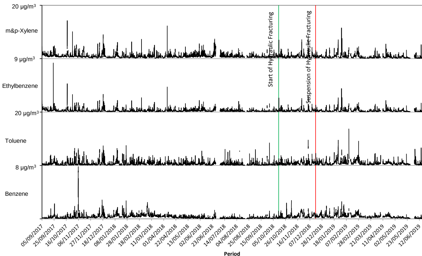
Figure 10. Time series plot of the BTEX 1-Hour Mean Concentrations ( \mu\text{g}/\text{m}^3 )
