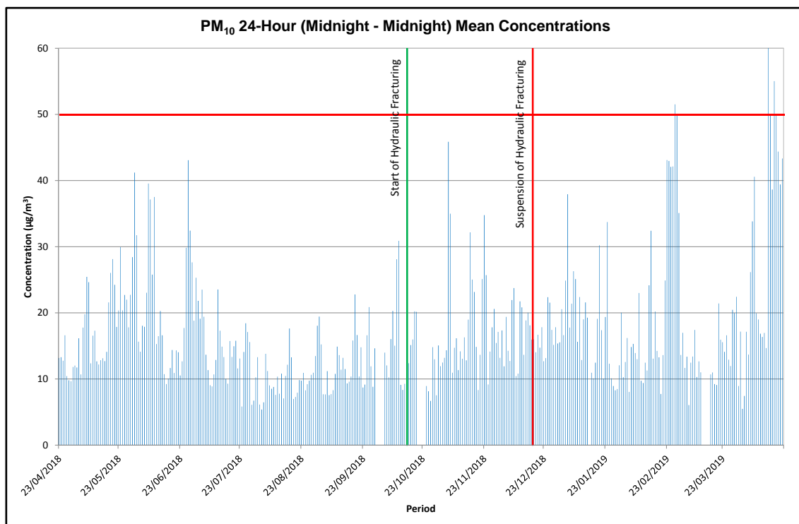
Figure 4. 24-hour (midnight-midnight) mean \text{PM}_{10} concentrations at the monitoring site
