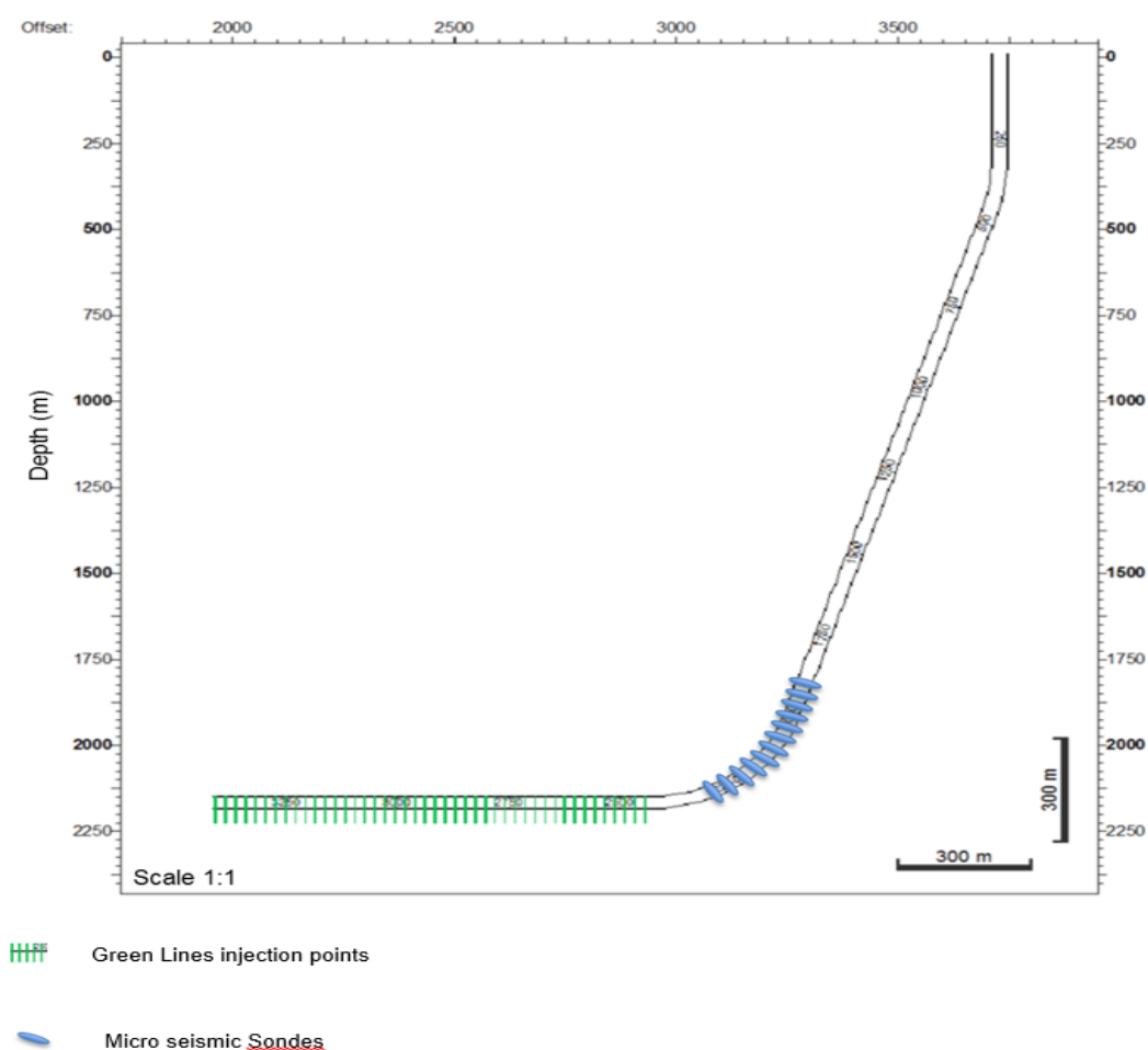
Figure 3: Illustrative figure of downhole micro seismic geophones
