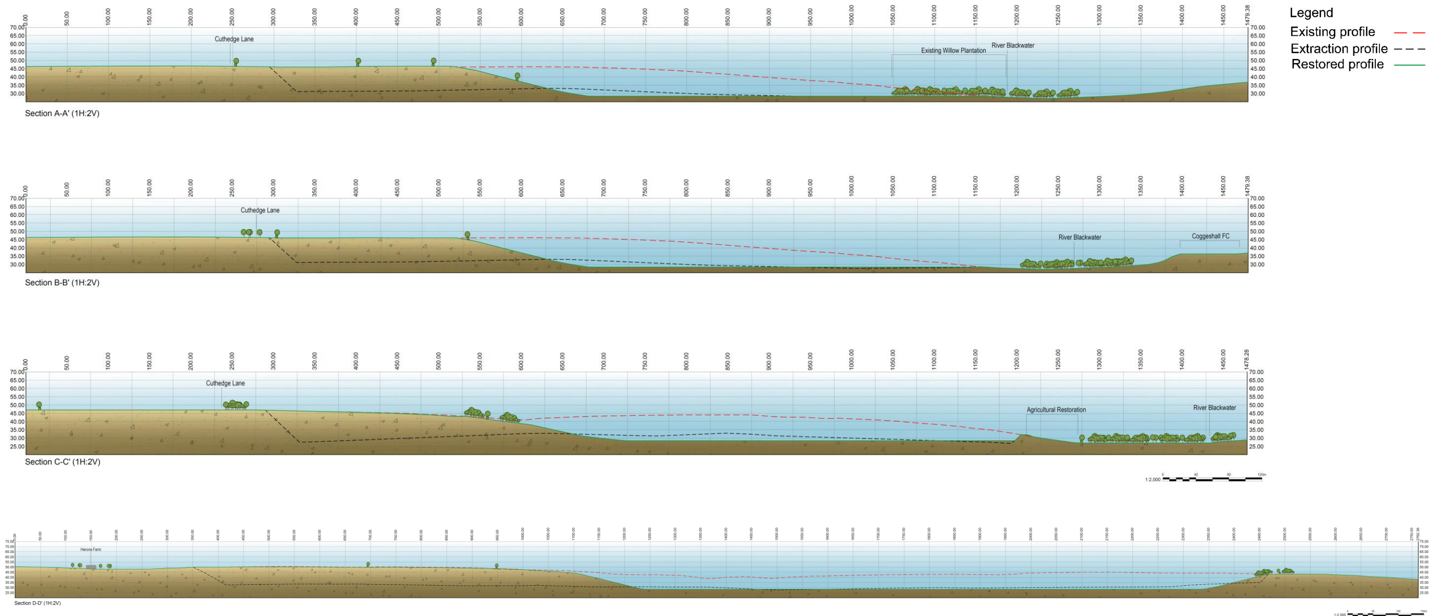
Cross sections through the restoration scheme.
